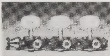
European classic style machine heads — mechanically identical to EMG but brass hand engraving on "gun metal" black background. Pearlloid buttons, plastic rollers, with lyre. Post hole spacing 70mm.
